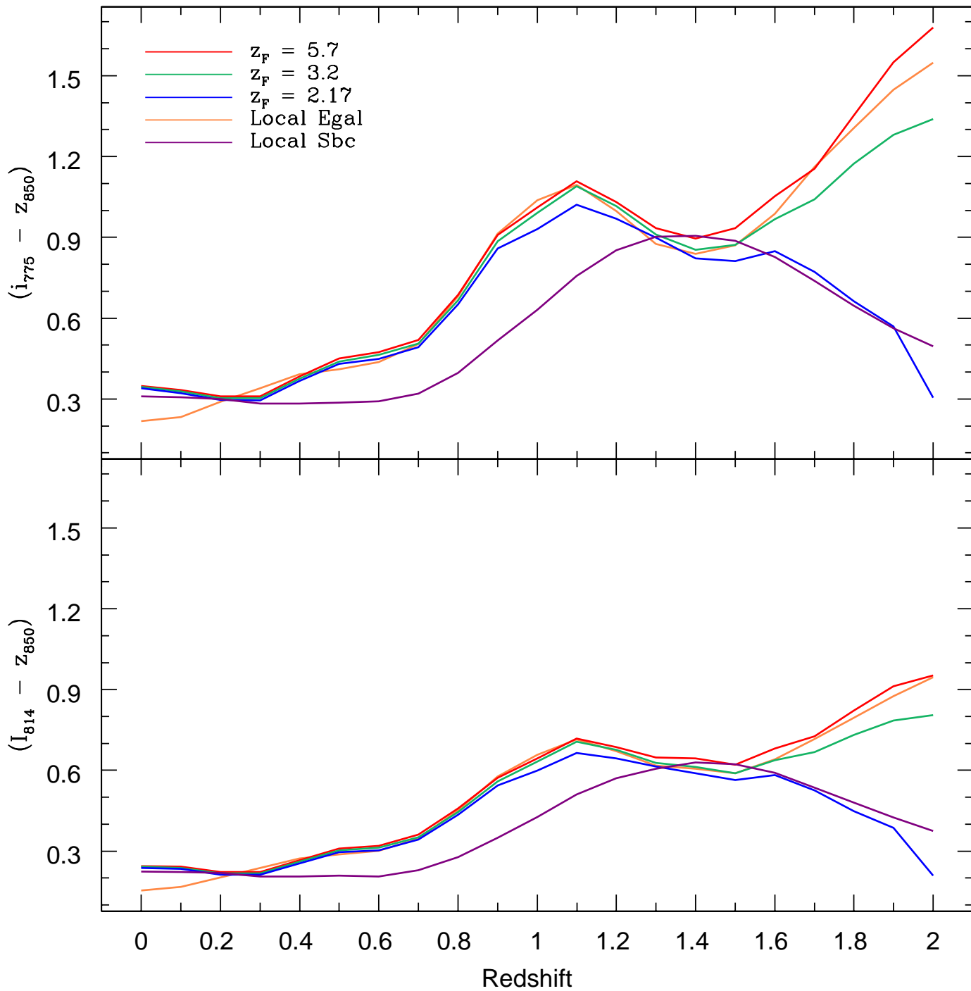
Models are BC03 SSP, Solar Metallicity
